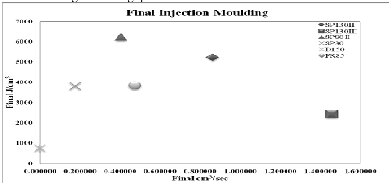
Figure 9. Sheet Metal processing: SEC Vs Flow Rate.
