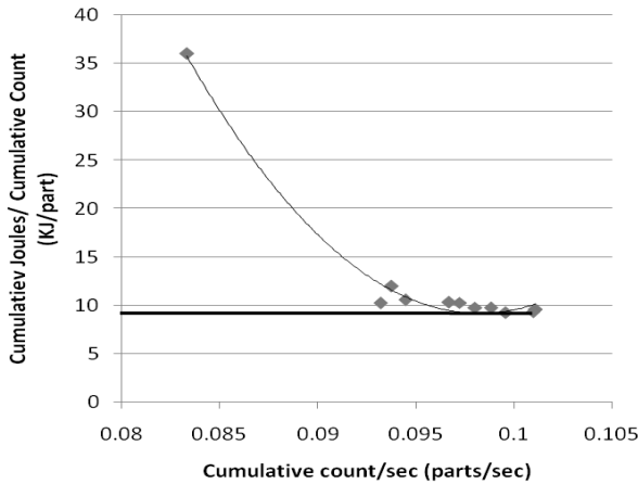
Figure 10. Electro-Discharge Machining: SEC Vs Flow Rate.
